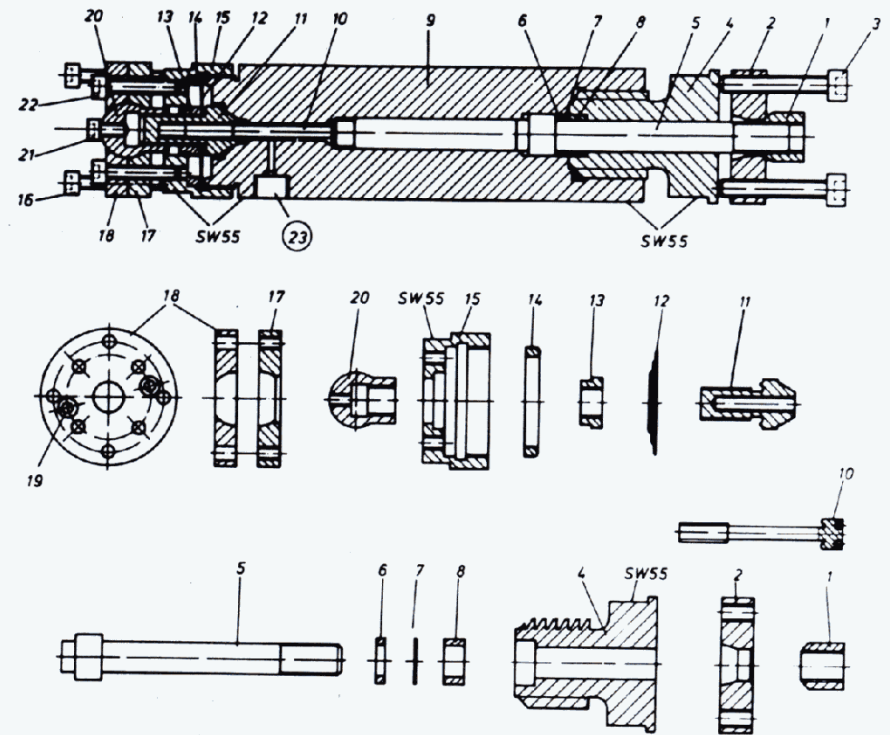
Fig. 3. High-pressure autoclave – closed system. (1) Hexagonal nut; (2) draw plate; (3) allen screw; (4) screwed fitting; (5) sealing rod; (6) sealing ring; (7) sealing ring; (8) thrust collar; (9) autoclave body; (10) high pressure valve; (11) sealing cone; (12) steel diaphragm; (13) nut; (14) sealing ring; (15) screwed fitting; (16) allen screw; (17) pull plate; (18) push plate; (19) countersunk screw; (20) ball joint; (21) allen screw; (22) allen screw and (23) ammonia inlet screw fitting.
