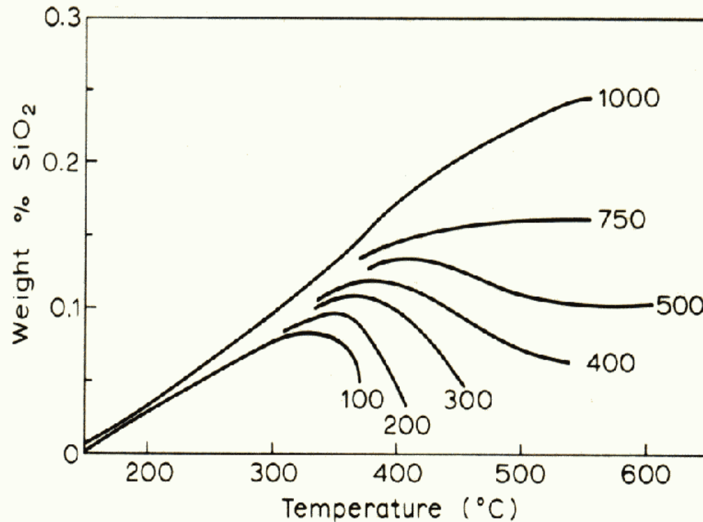
Fig. 2. The solubility of quartz in water at various pressures (in bars).
