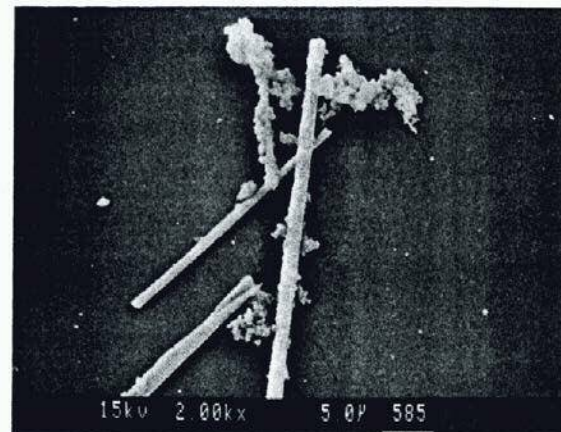
Fig. 3. SEM photograph of single monocrystalline AlN columns, direction of growth [001]; isothermal chemical transport, T = 600^\circ\text{C} , P = 2 kbar, x(\text{K})\text{Al} = 9\% and x(\text{NH}_3)\text{S} = 89\% .
