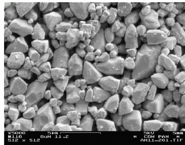
Figure 1. GaN crystals obtained in a synthesis process under the following conditions: T = 550^\circ\text{C} , p = 5 kbar, \text{Ga}:\text{LiNH}_2:\text{NH}_3 = 1:2:20 .
