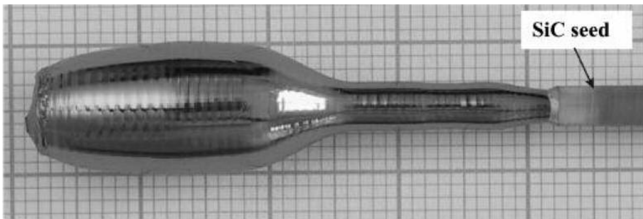
Fig. 2 ^{29}\text{Si} crystal grown by mini-CZ technique from the 4g charge using SiC seed.
