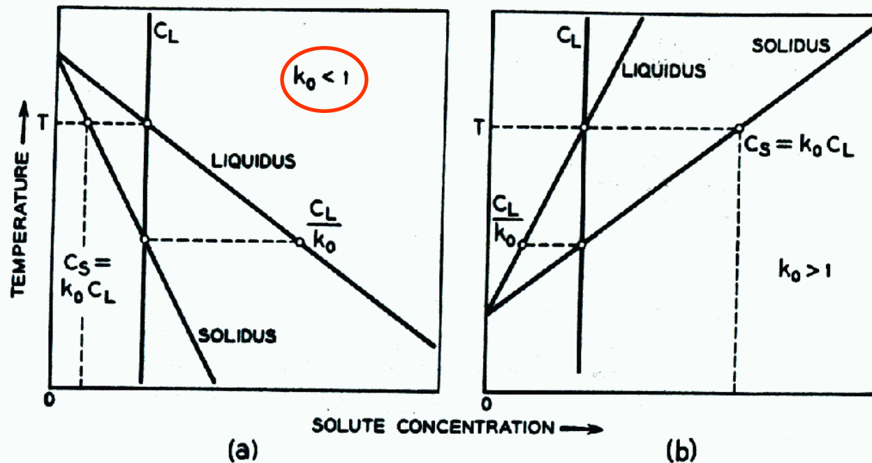
FIG. 1. Portions of constitutional diagrams in which the freezing point of the solvent is, (a) lowered, (b) raised, by the solute.
