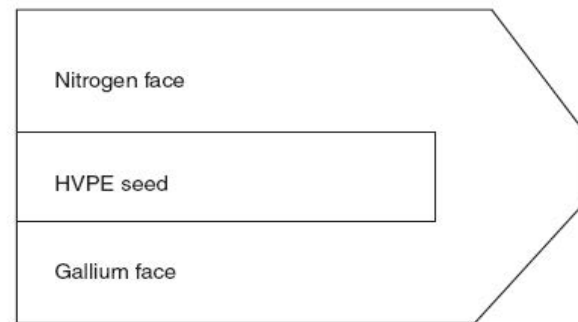
Fig. 3. (a) Optical transmission (Xenon lamp) image of the cross-section of an as-grown ammonothermal GaN crystal and (b) schematic drawing of the crystal in (a) with 200 \mu\text{m} thick HVPE GaN seed.
