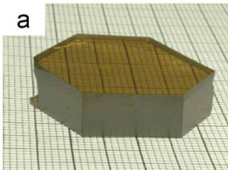
Fig. 2. The thick 1-in AMMONO-GaN crystal (a) and 11 mm \times 22 mm non-polar ( m -plane) substrate cut out of this crystal (b).
