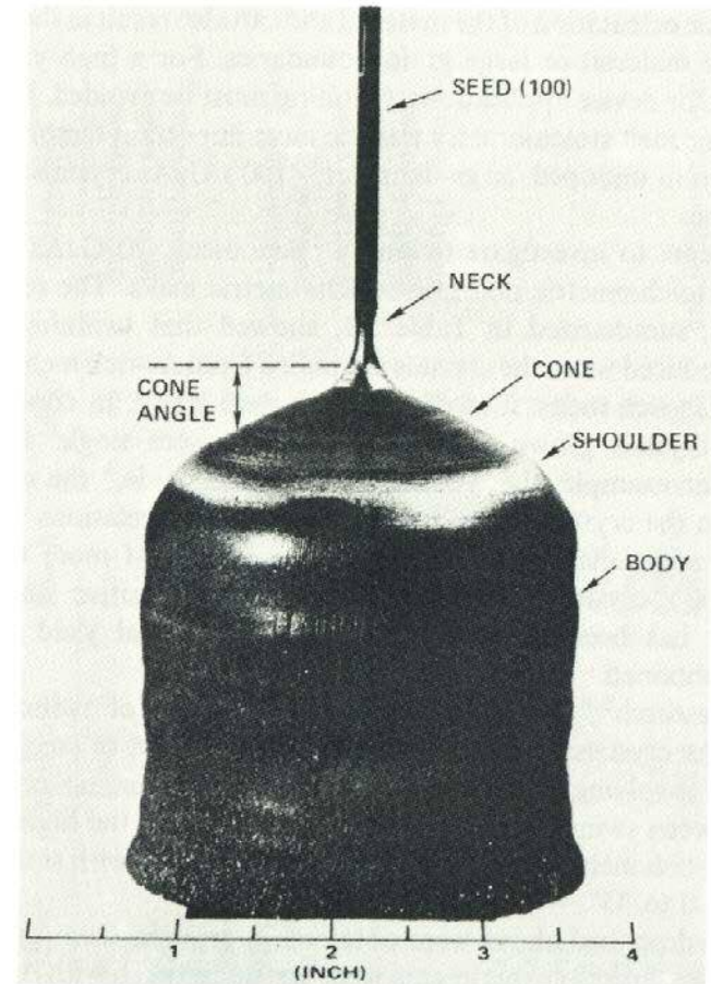
Figure 2.3 LEC GaAs (100) crystal and seed
