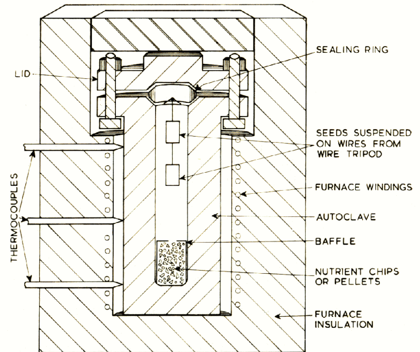
FIG. 14.6. Typical arrangement of furnace and autoclave for hydrothermal growth of crystals.
