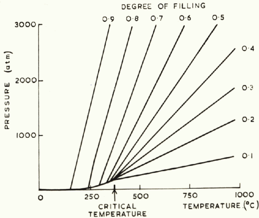
FIG. 14.10. P-T curves for water for various initial degrees of filling, after Kennedy (1950a).
