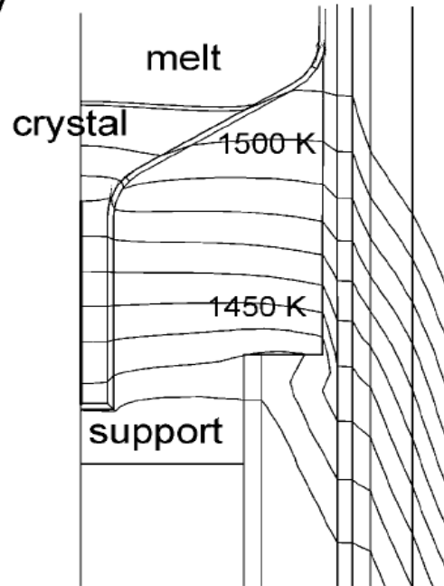
(b) \lambda_{\text{support}} = 5 \text{ W/mK} max. \sigma_{\text{VM}} = 1.93 \text{ MPa}
