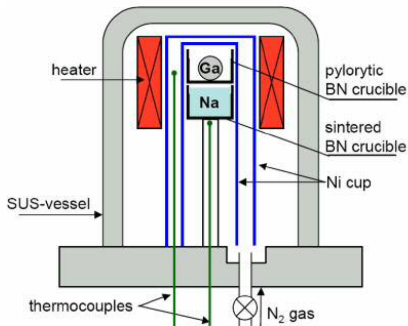
Fig. 1 Schematic drawing of the apparatus used for the crystal growth. A pyrolytic BN (or sintered BN) crucible containing Ga was placed on a sintered BN crucible containing Na. These crucibles were covered with a Ni cap.
