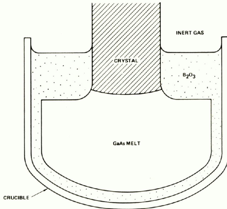
Figure 2.2 LEC crucible configuration during growth
