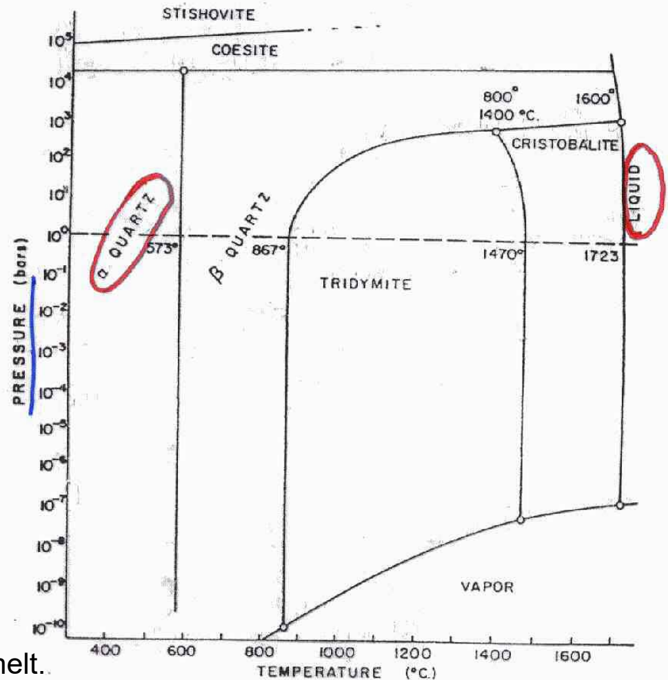
Figure 27. P-T diagram for system \text{SiO}_2 drawn to scale. From Roy and White (1975).
